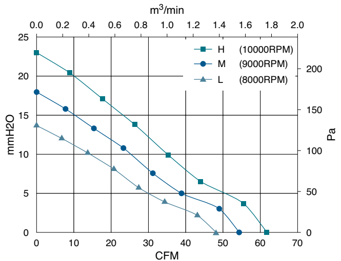
60x60x38mm DC Industry Fan P/Q Curves (At rated speed)
